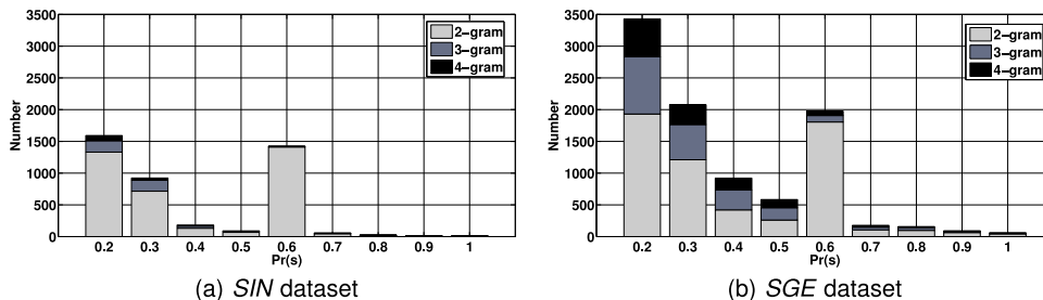
Fig. 7. The distributions of n -grams by Pr(s) for n = 2, 3, 4 .
