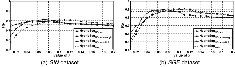
Fig. 6. The impact of \lambda on HybridSeg NGram on the two data sets.
