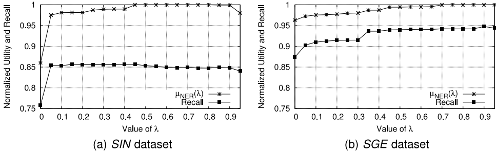
Fig. 5. Re and normalized \mu_{NER}(\lambda) values of HybridSeg NER with varying \lambda in the range of [0, 0.95] .
