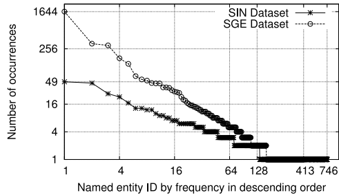
Fig. 4. Frequency distribution of the annotated NEs.
