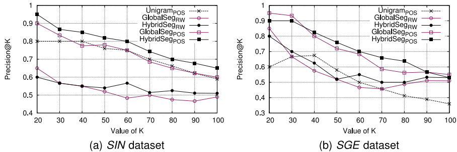
Fig. 8. Precision@K on two data sets.
