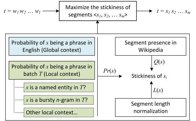
Fig. 2. HybridSeg framework without learning from pseudo feedback.
