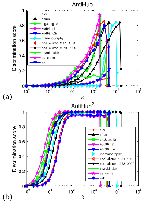
Fig. 7. Discrimination of AntiHub and AntiHub 2 scores.
