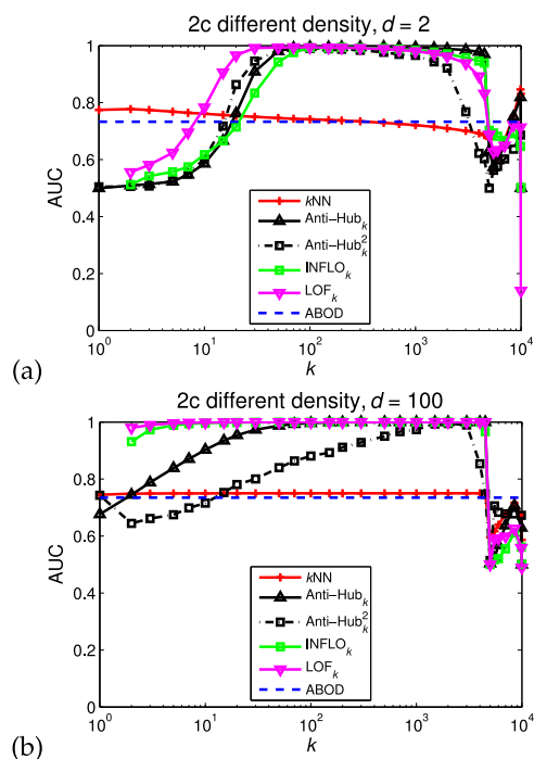
Fig. 8. Results for synthetic data with two clusters.
