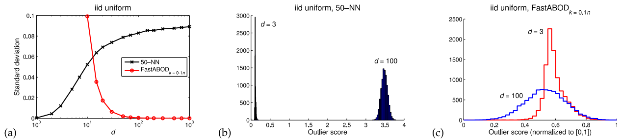
Fig. 1. Outlier scores versus dimensionality d for uniformly distributed data in [0, 1]^d : (a) Standard deviation; (b) Histogram of 50-NN scores; (c) Histogram of normalized ABOD scores.
