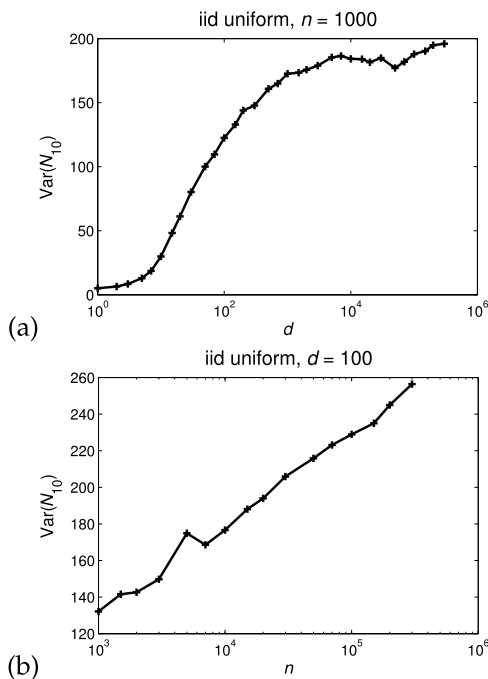
Fig. 6. Observed \text{Var}(N_{10}) on iid uniform random data for (a) n = 1,000 , varying d ; (b) d = 100 , varying n .
